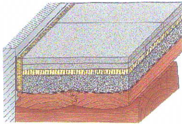
Timber floor
